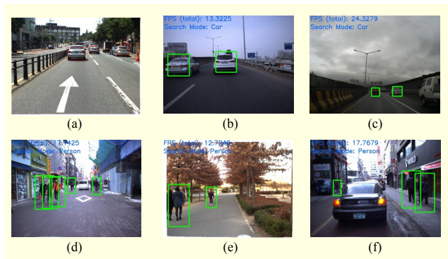
Fig. 6. Vehicle recognition results for (a) urban road, (b) highway, and (c) highway in rain. Pedestrian recognition results for (d) downtown street, (e) residential street, and (f) urban road.
